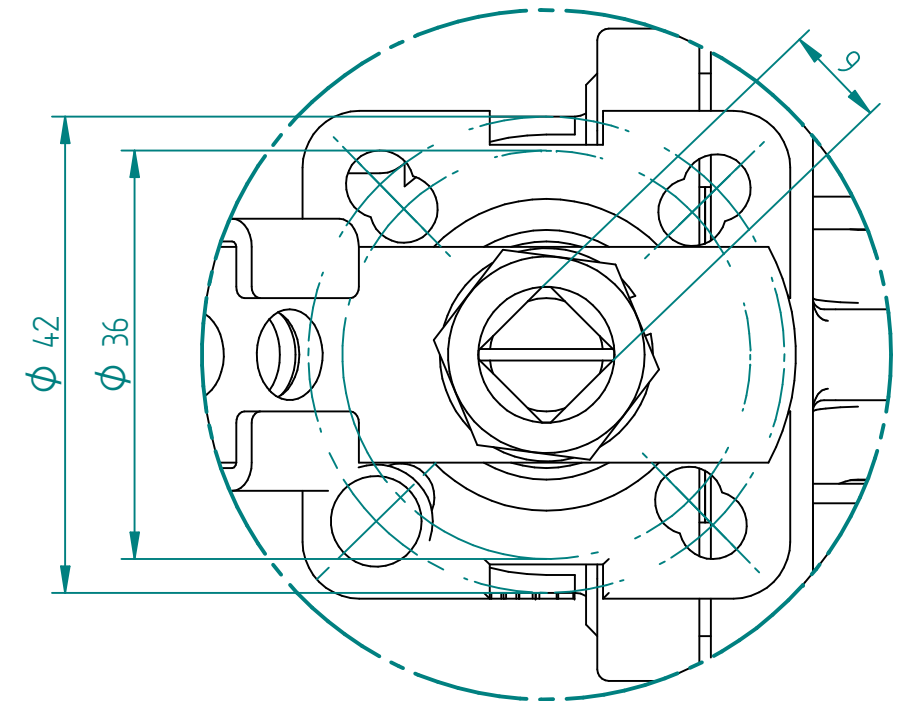
DETAIL A ISO 5211 Mounting Pad 1,5:1
