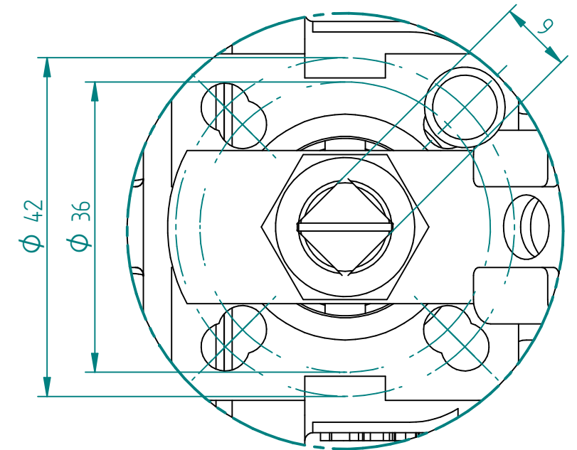
DETAIL A ISO 5211 Mounting Pad 1,5:1
