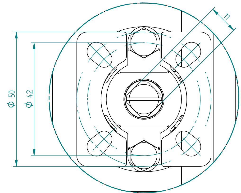
DETAIL A ISO 5211 Mounting Pad 1,5:1
