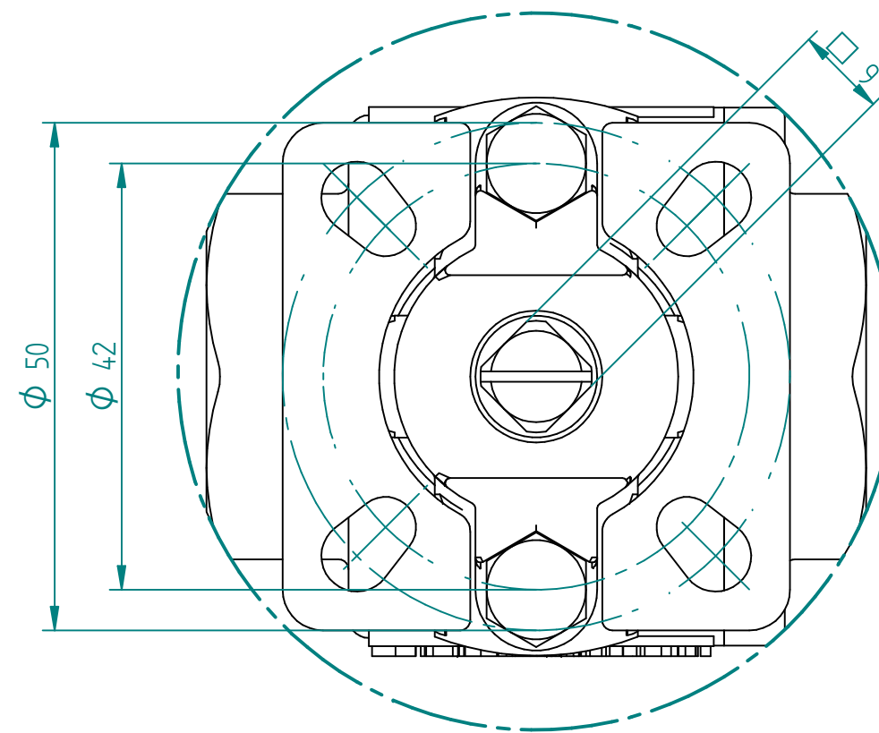
DETAIL A ISO 5211 Mounting Pad 1.5:1
