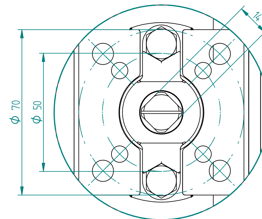
DETAIL A ISO 5211 Mounting Pad 1:1
