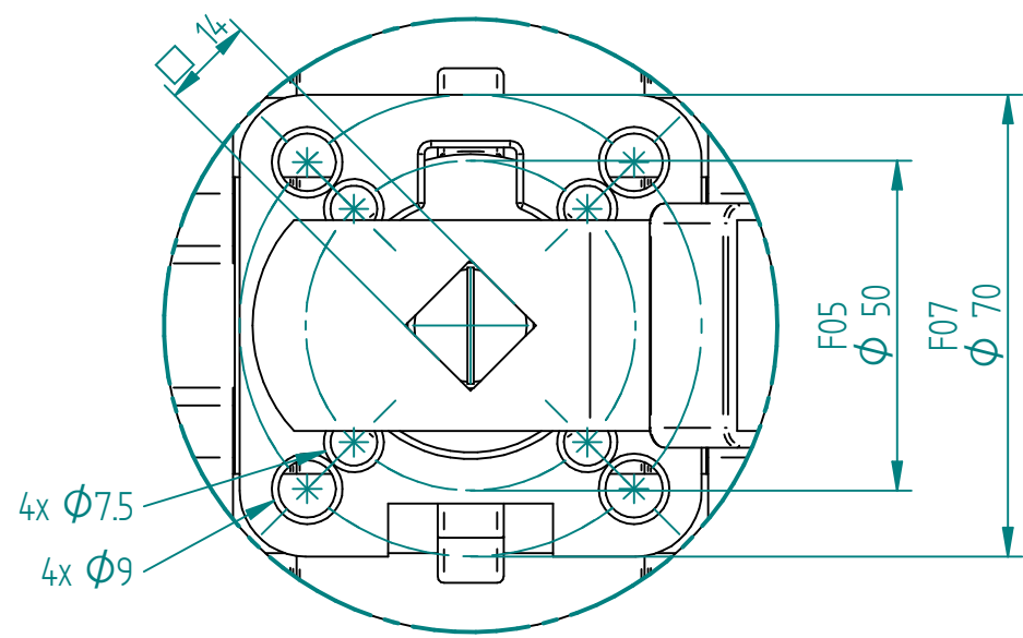
DETAIL A
