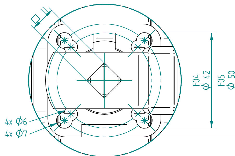
DETAIL A
