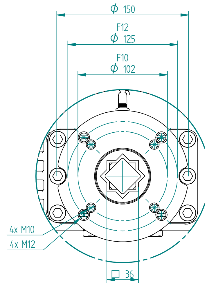
DETAIL A
