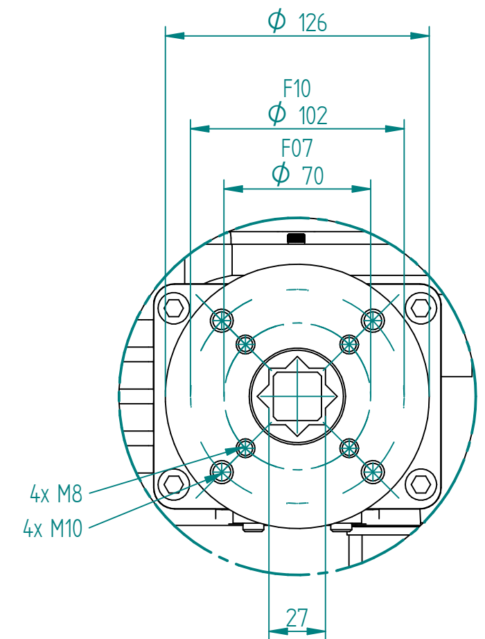
DETAIL A
