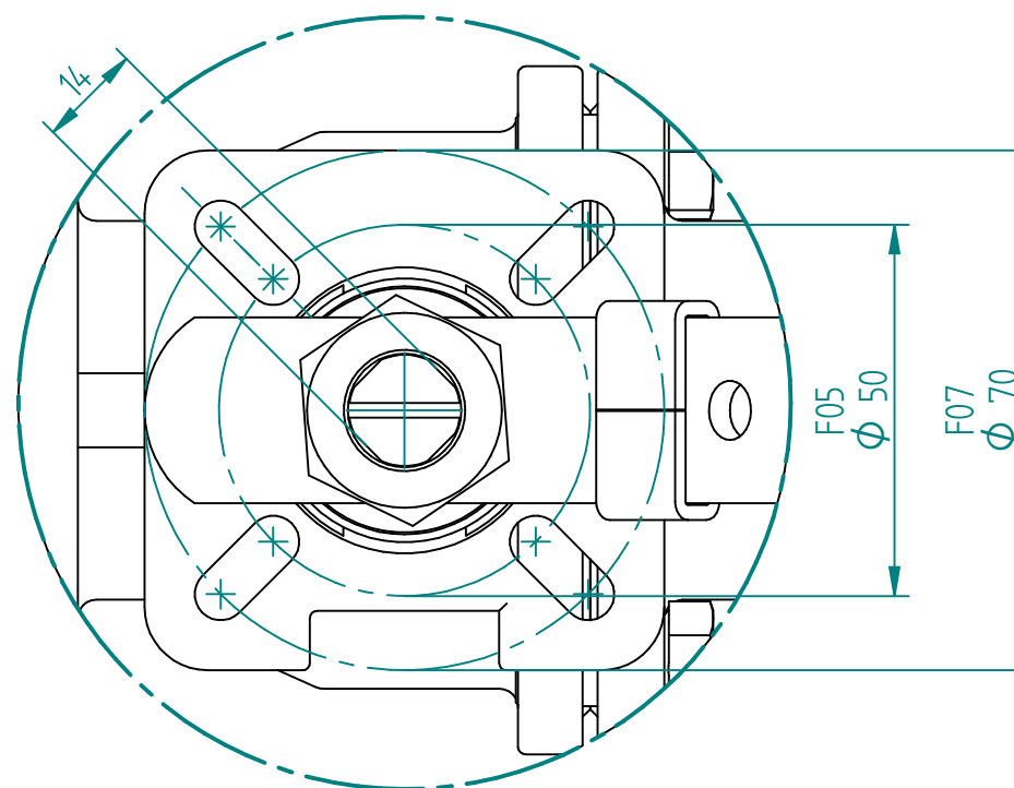
DETAIL A
