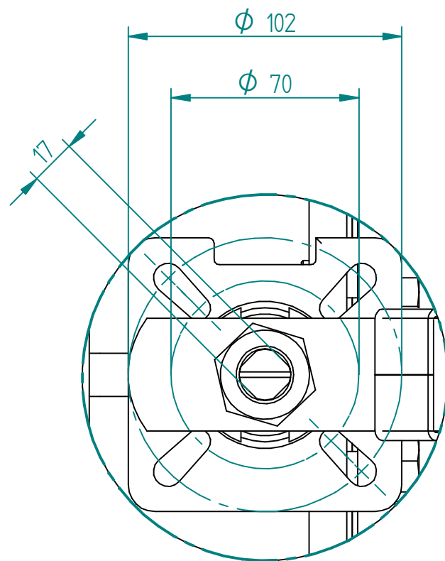
DETAIL A
