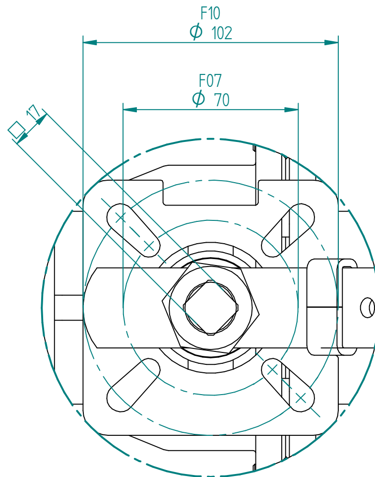
DETAIL A
