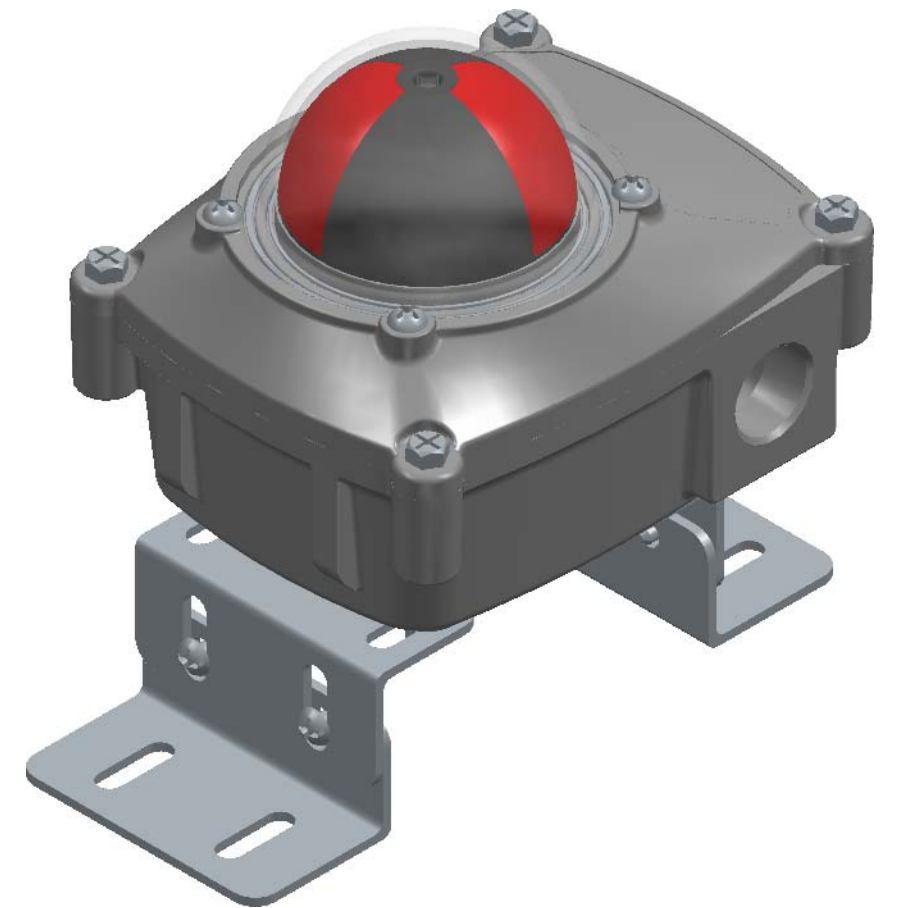
Switchbox, Aluminium alloy + epoxy coated body dome type open & close indicator, 2xSPDT, IP68 304SS bolts/shaft/universal bracket, M20*1.5
