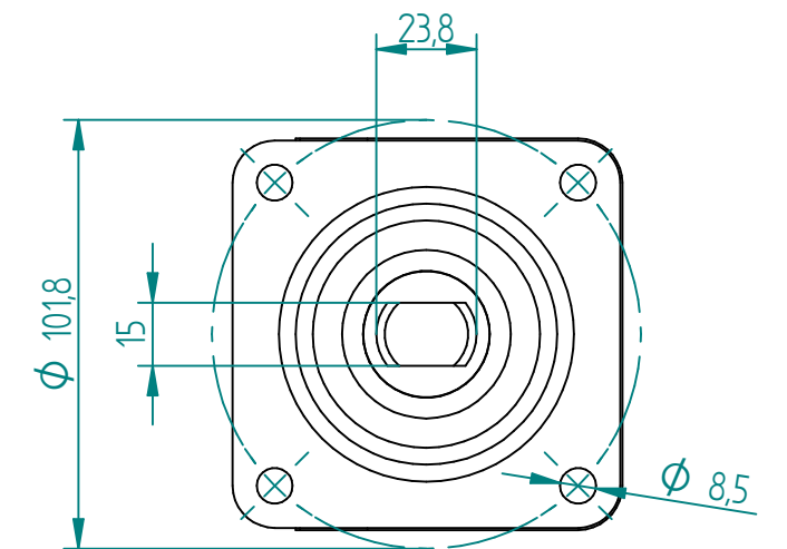
1:2 Dual Pattern ISO 5211 Mounting Pad
