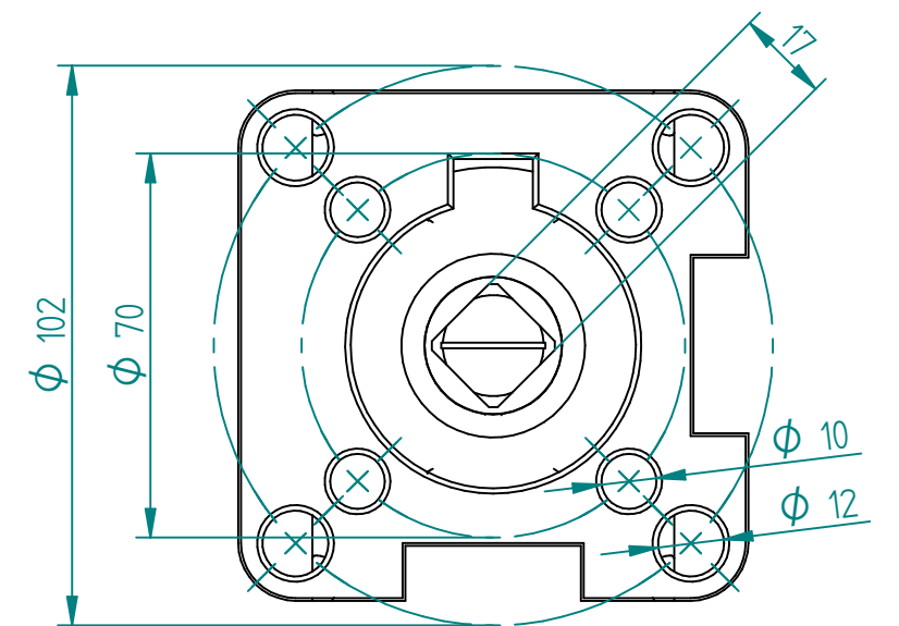
Dual Patern 1:15 ISO 5211 Mounting Pad
