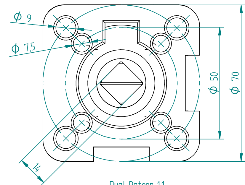
Dual Patern 1:1 ISO 5211 Mounting Pad
