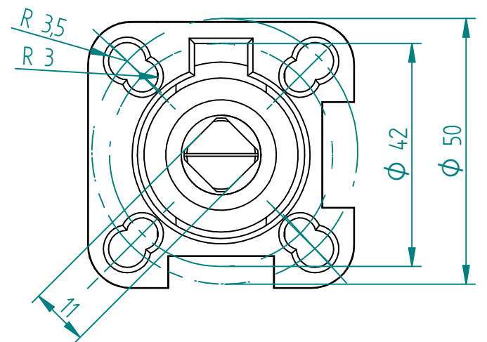
Dual Patern 1:1 ISO 5211 Mounting Pad
