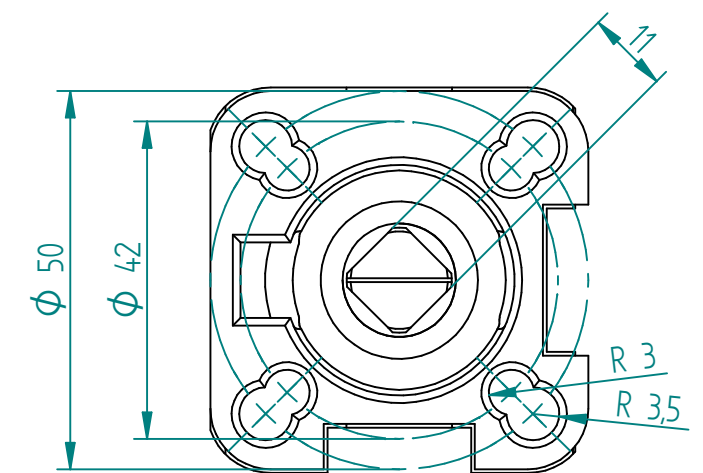
Dual Patern 1:1 ISO 5211 Mounting Pad
