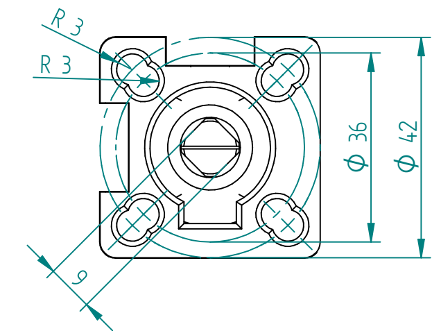
Dual Pattern 1:1 ISO 5211 Mounting Pad
