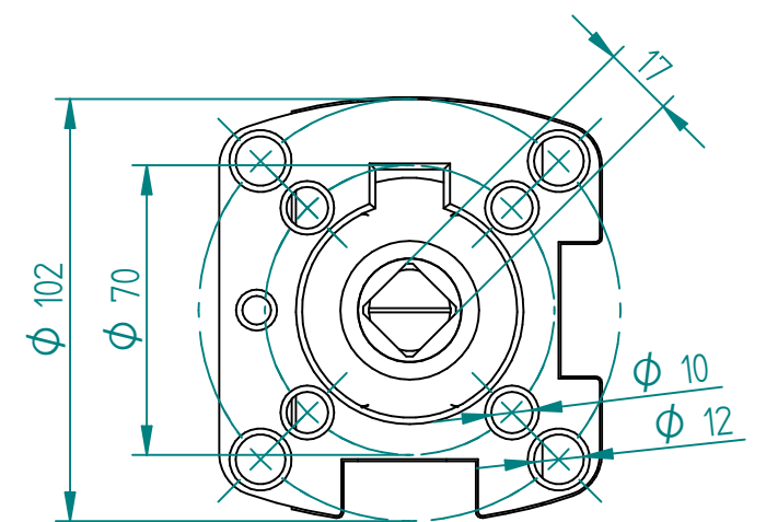
Dual Pattern 1:2 ISO 5211 Mounting Pad
