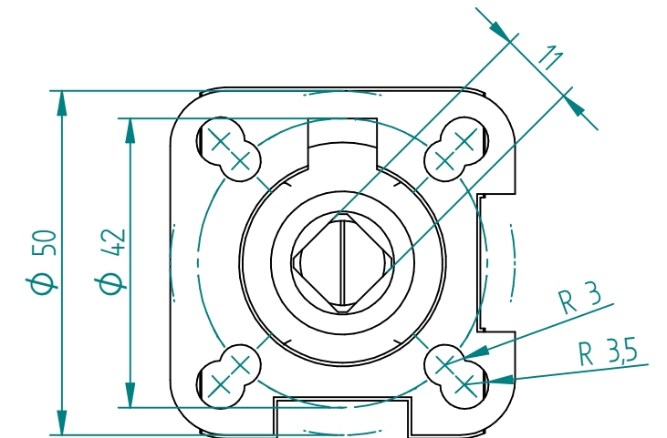
1:1 Dual Pattern ISO 5211 Mounting Pad
