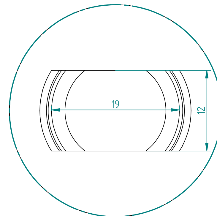
DETAIL A 3:1
