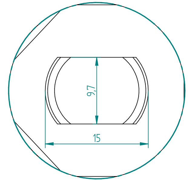
DETAIL A 3:1
