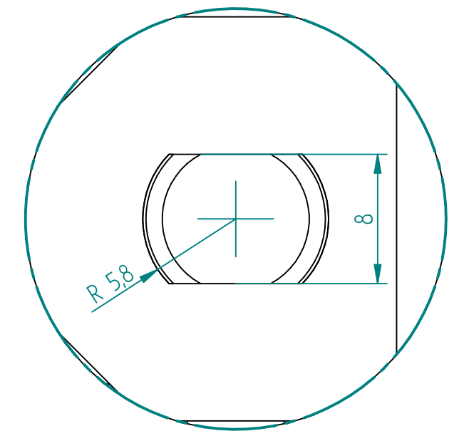
DETAIL A 3:1
