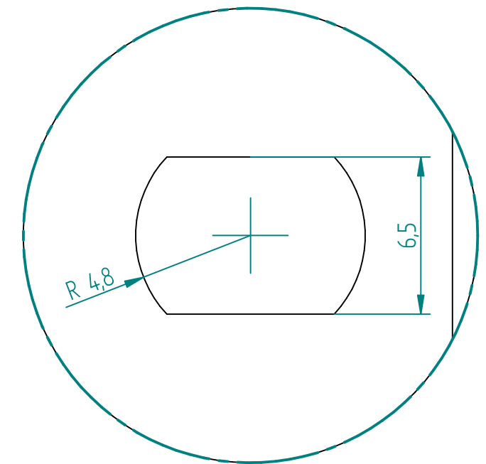
DETAIL A
