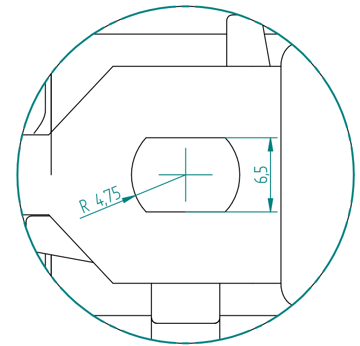
DETAIL A 3:1
