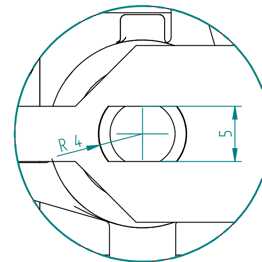
DETAIL A 3:1
