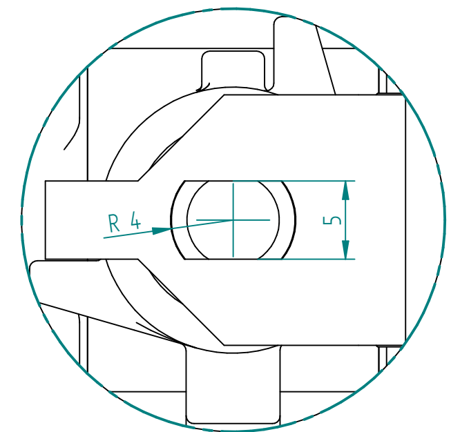
DETAIL A 3:1
