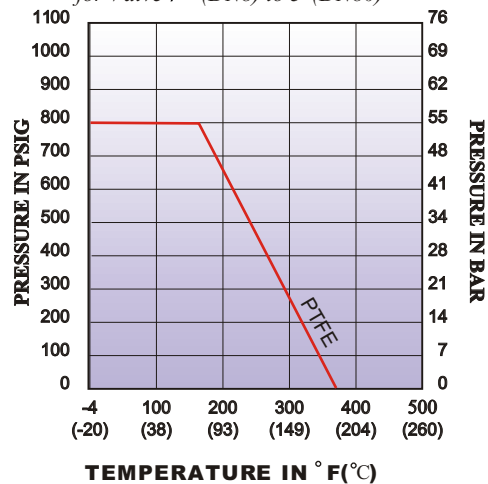
Pressure Vs. Temperature Chart for Valve Y # (DN8) to 3"(DN80)
