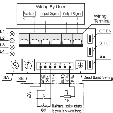
SF-ZC Servo-Controller
