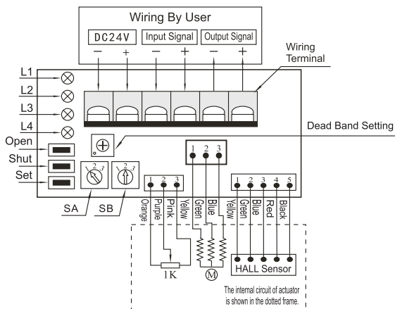
SF-LC/DC24V Servo-Controller
