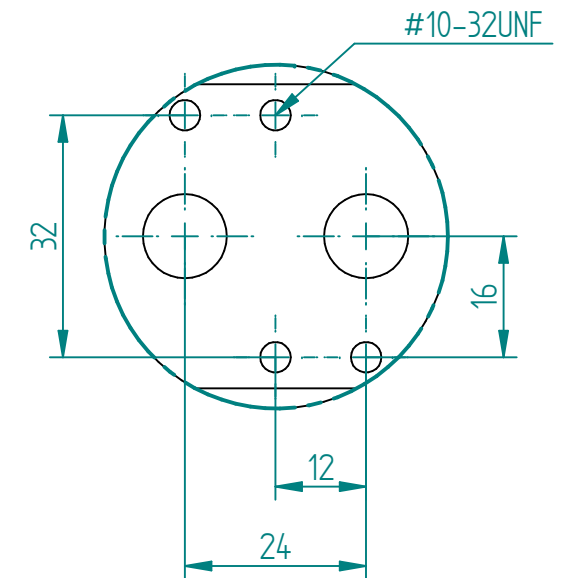
DETAIL A 1:1 NAMUR SOLENOID MOUNTING
