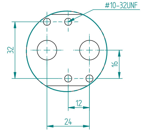
DETAIL A 1:1 NAMUR SOLENOID MOUNTING
