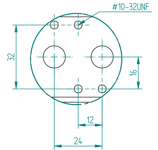
DETAIL A 1:1 NAMUR SOLENOID MOUNTING
