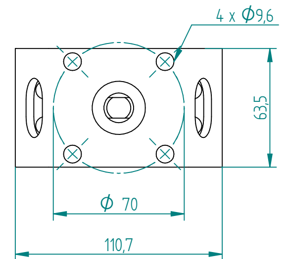
1:2 Mounting Plate
