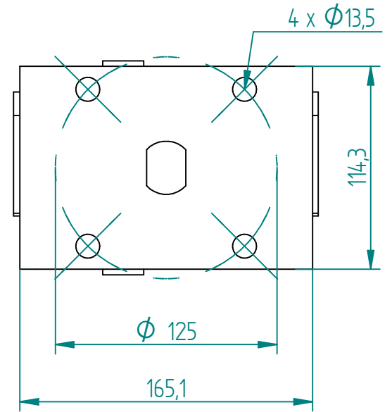
1:3 Mounting Plate
