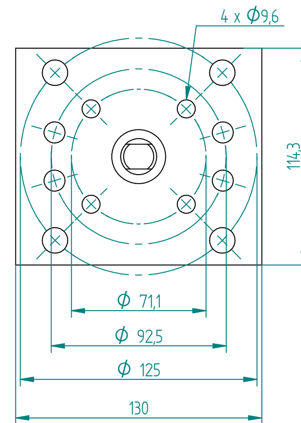
1:2 Mounting Plate
