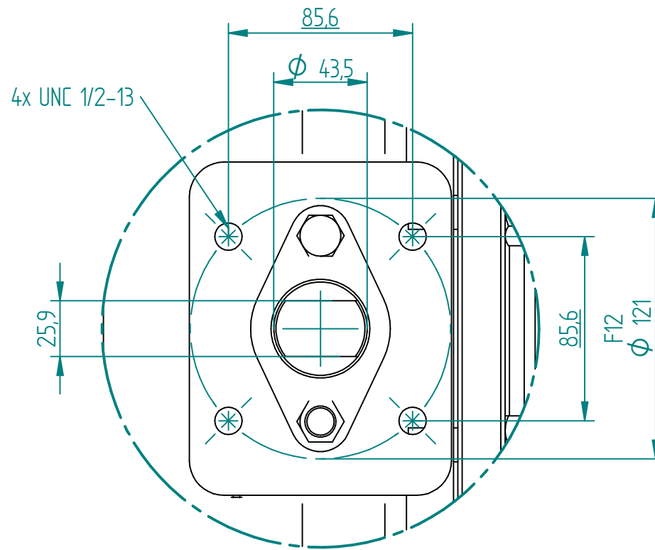
DETAIL A
