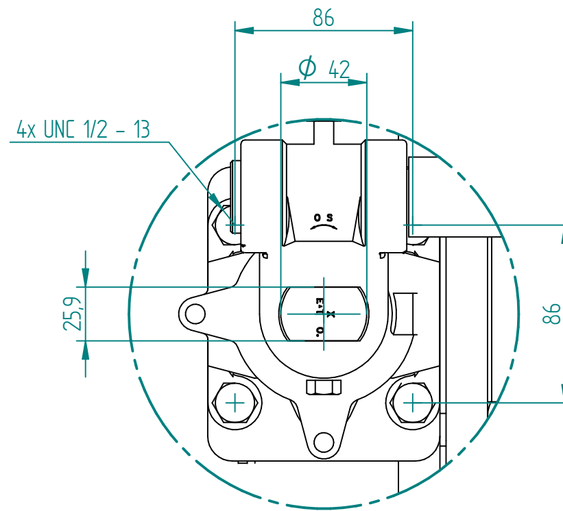
DETAIL A
