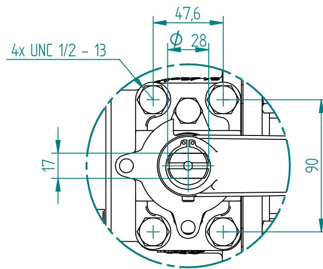
DETAIL A
