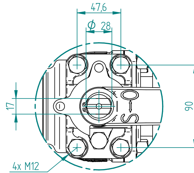
DETAIL A
