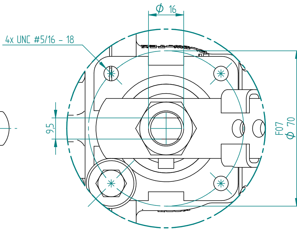
DETAIL A
