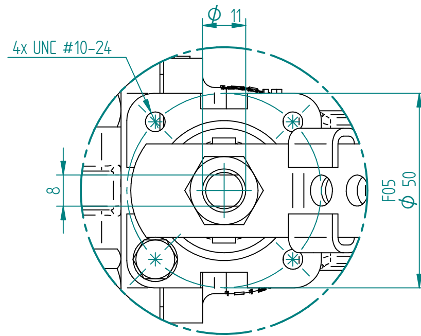
DETAIL A
